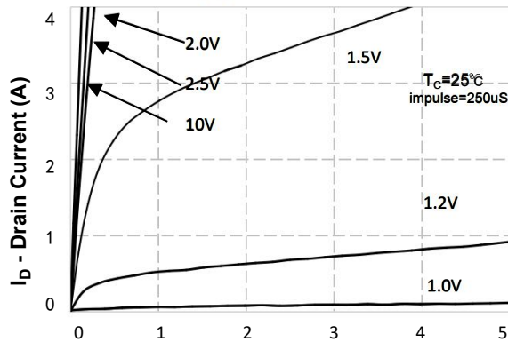
Figure 1. On-Region Characteristics
