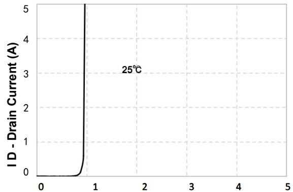
Figure 2. Transfer Characteristics
